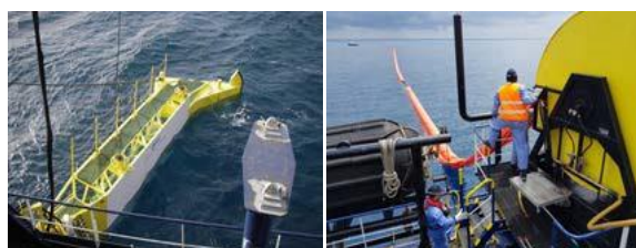
Sweeping arm
